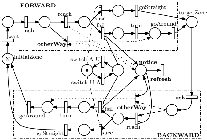
Fig. 7: Centralized architecture.
